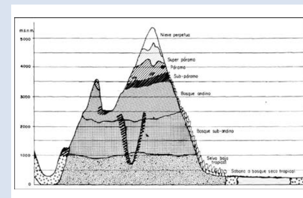
Figure 1. Ecosystems and altitudes in El Cocuy National Park
